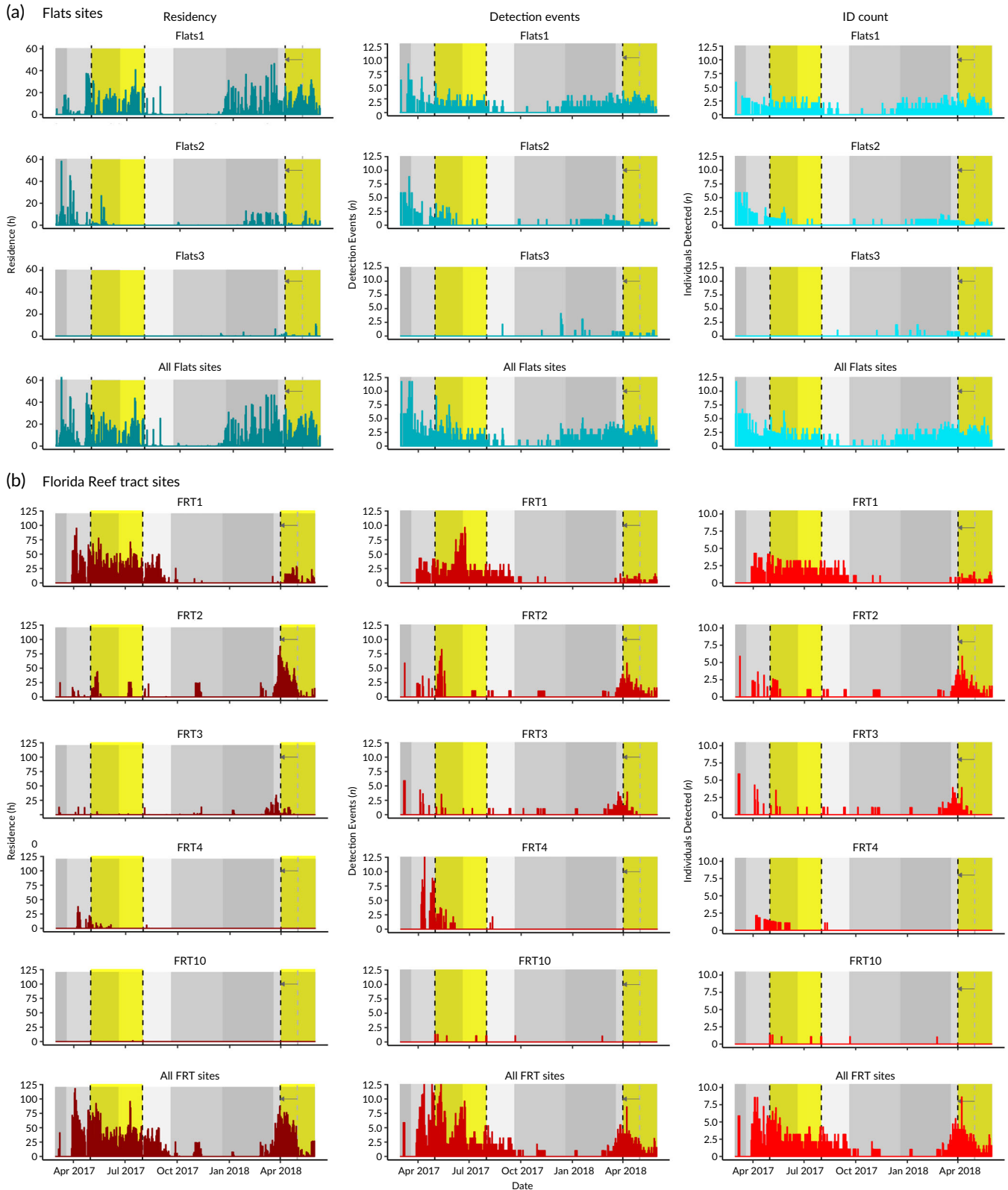
FIGURE 2 (a) Corrected Trachinotus falcatus space use including residency (h), detection events (n), and individual permit detected (ID count n) at flats sites (■) and (b) Florida Reef Tract sites (■), from March 2017 to June 2018. ■, The time periods where T. falcatus harvest was prohibited in the special permit zone (SPZ), which was May through July in 2017, extended to include April in 2018. Only sites that have \geq 10 total detection events are shown. Season: (■) Winter, (□) Spring, (□) Summer, and (□) Fall. (■) Closed Harvest Period
