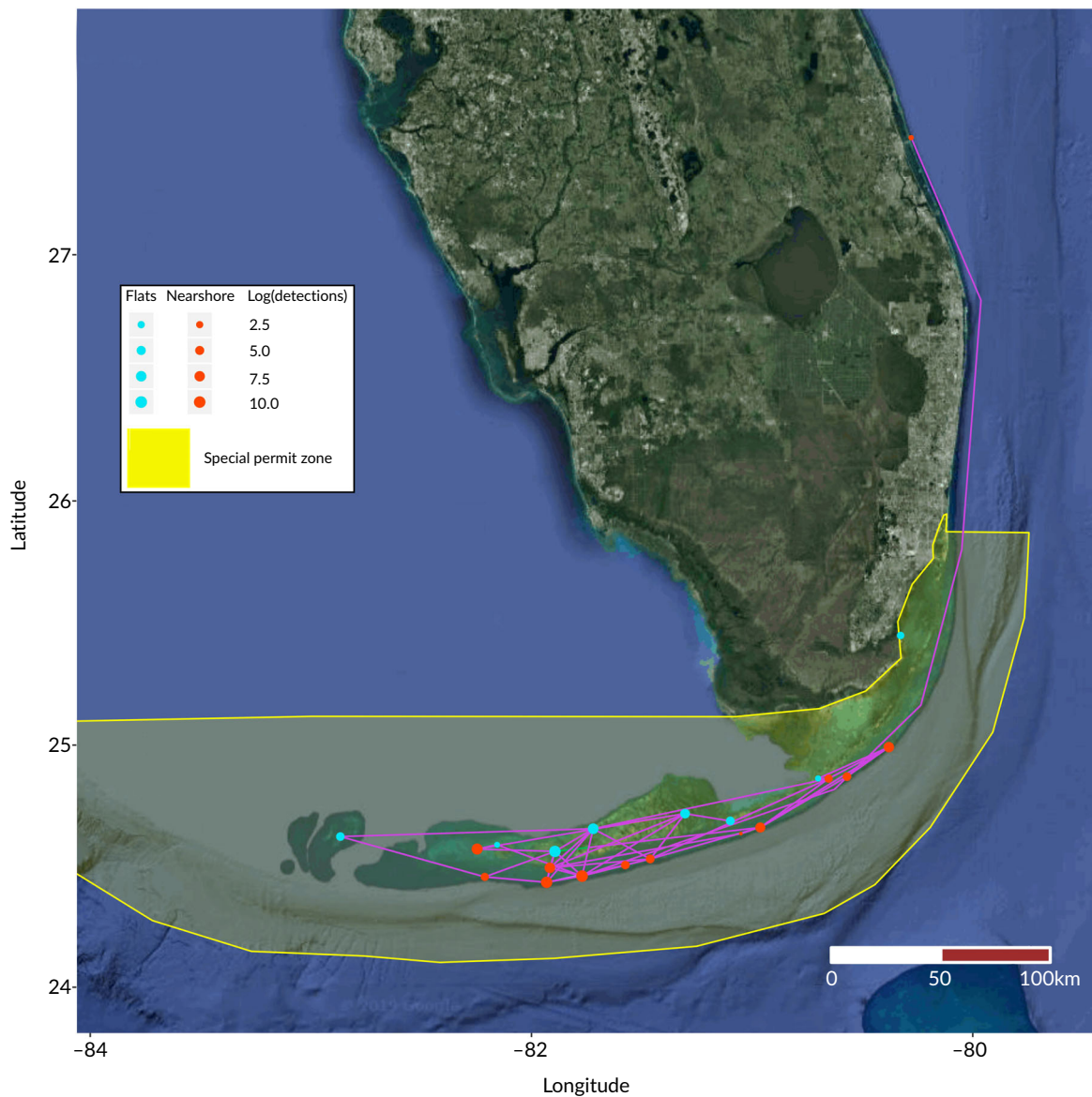
FIGURE 1 Map of Trachinotus falcatu detections at general locations, categorised by flats (●) and nearshore (●, includes the Florida reef tract and shipwreck) sites. The size of the circle indicates the log+1 transformed total number of T. falcatu detections at each location. —, Trachinotus falcatu movements between sites; □, the special permit zone (SPZ), which extends south from Cape Florida in the Atlantic Ocean to Cape Sable in the Gulf of Mexico, including state and federal waters
